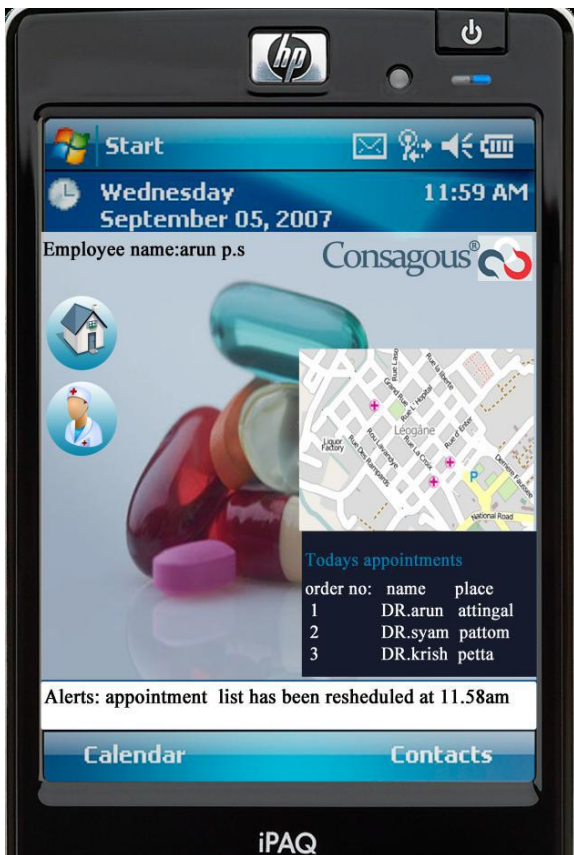
User interface
