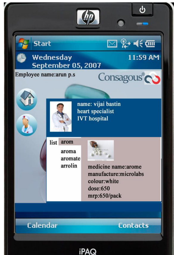
Doctors interface
